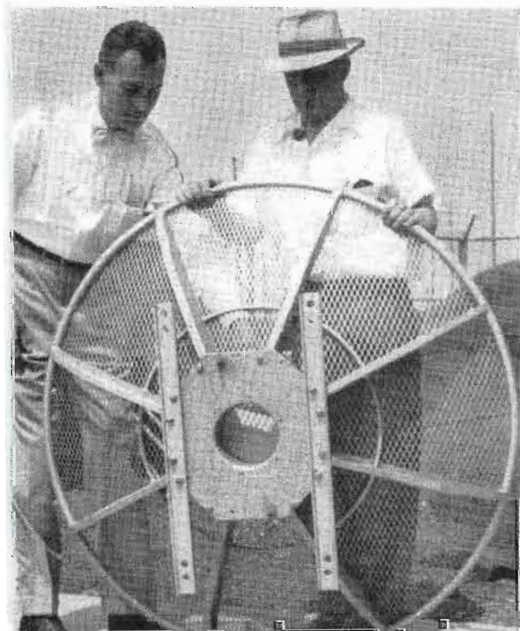
Left: RCA engineers Williamson and Sadler inspect one of the microwave parabolic antennas used in the Riverhead-to-New York relay system.
